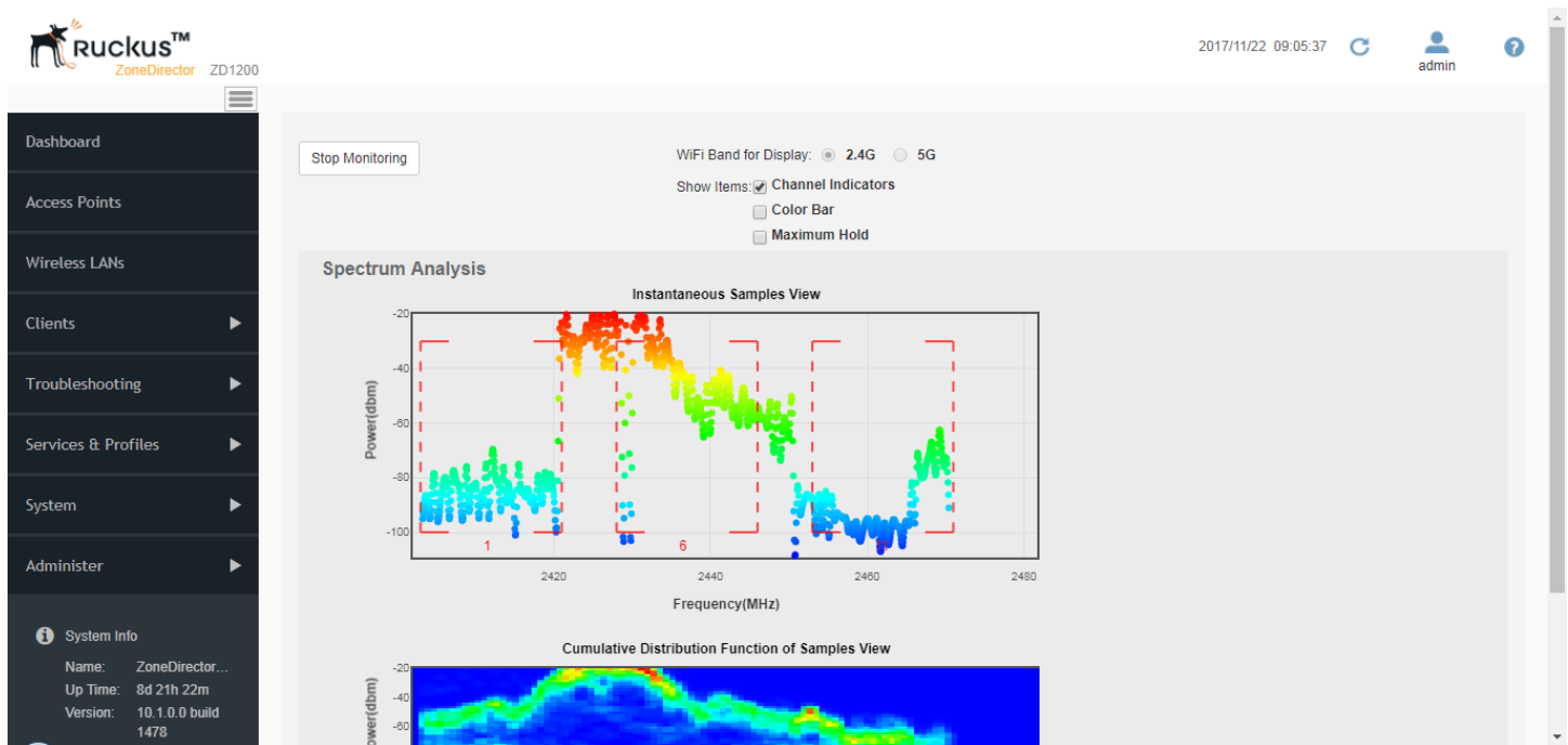
FIGURE 269 Performing Spectrum Analysis on the 2.4 GHz radio
